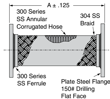
AF-21-FF FLXFL FLEX CONNECTORS
