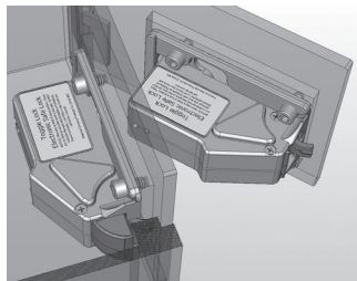
TOGGLE LOCK
