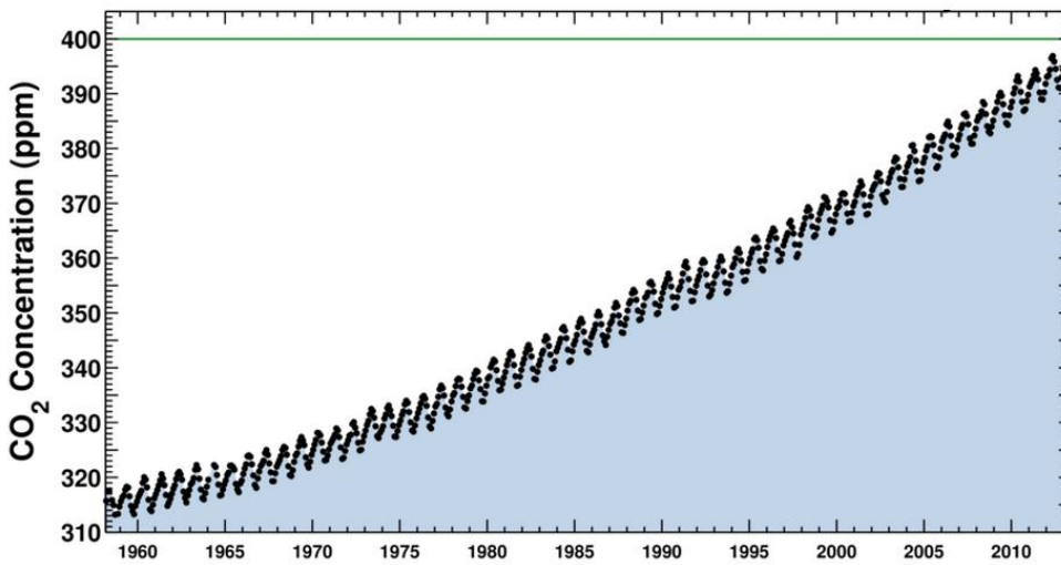
Figure 1: Carbon dioxide concentration at Mauna Loa Observatory
