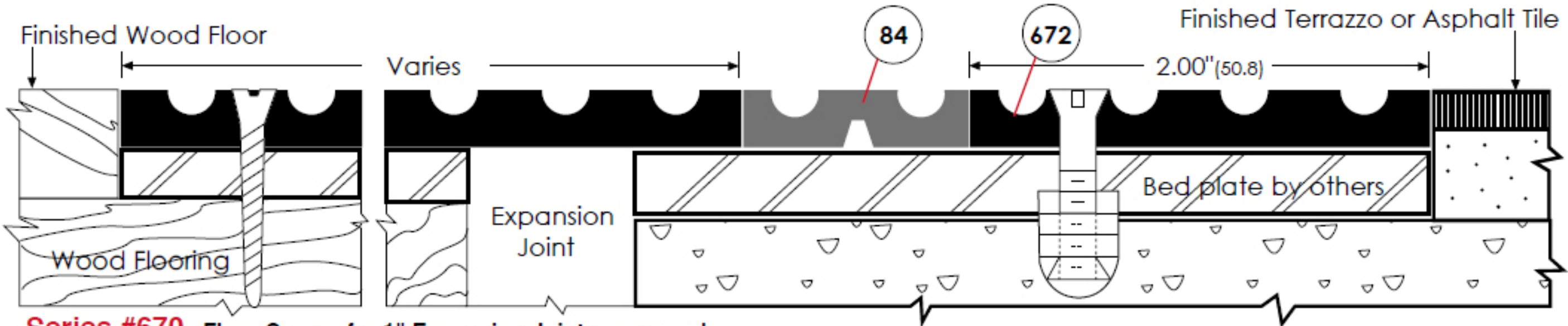
Series #670 Floor Covers for 1" Expansion Joints, recessed
