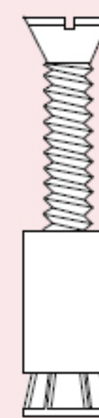
c MSLA-10 Anchor with machine screw 10/24
