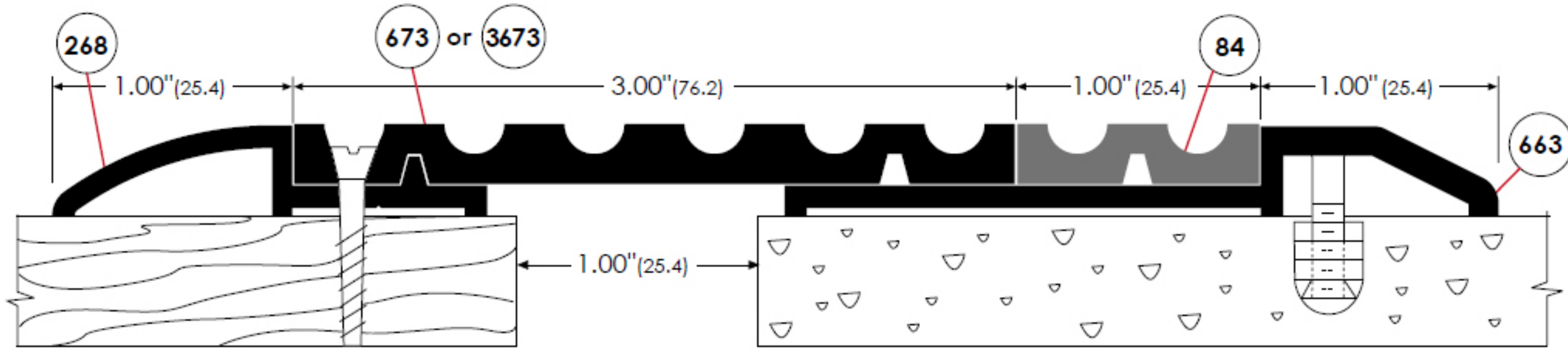
Series #671 Floor Covers for 1" Expansion Joints, surface
