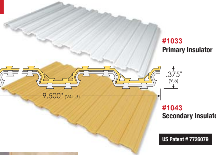
Wall Framing #1033 / #1043
