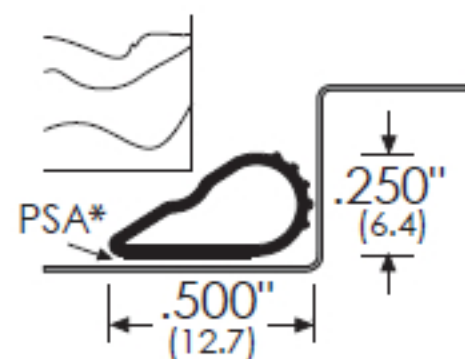
#188S-Bk #188S-Br #188S-CI #188S-Gy #188S-Wh #188 FS
