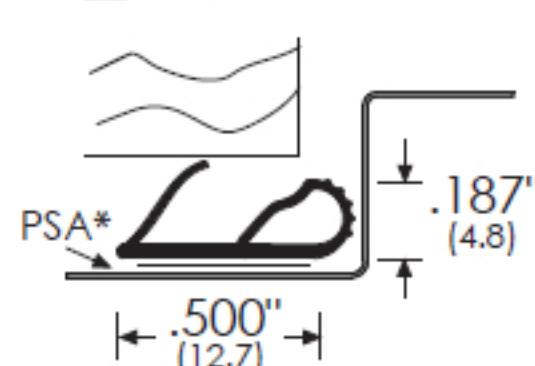
#8145S-Bk ZERO Compress-O-Matic®
