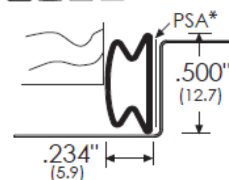
#8216S-Bk .500" For metal frame #8218S-Bk .375" For wood frame
