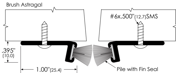
Surface Mounted Meeting Stile - Both Doors Active - Angle Pile Brush
