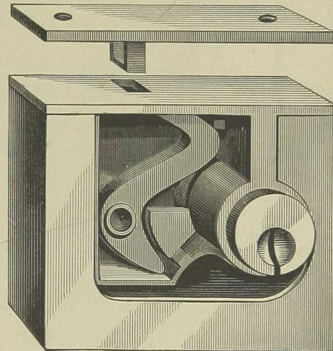
Tin Box Lock No. 151.
