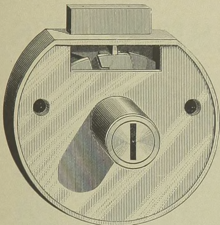
STANDARD RIM-FLUSH DRAWER LOCK.
