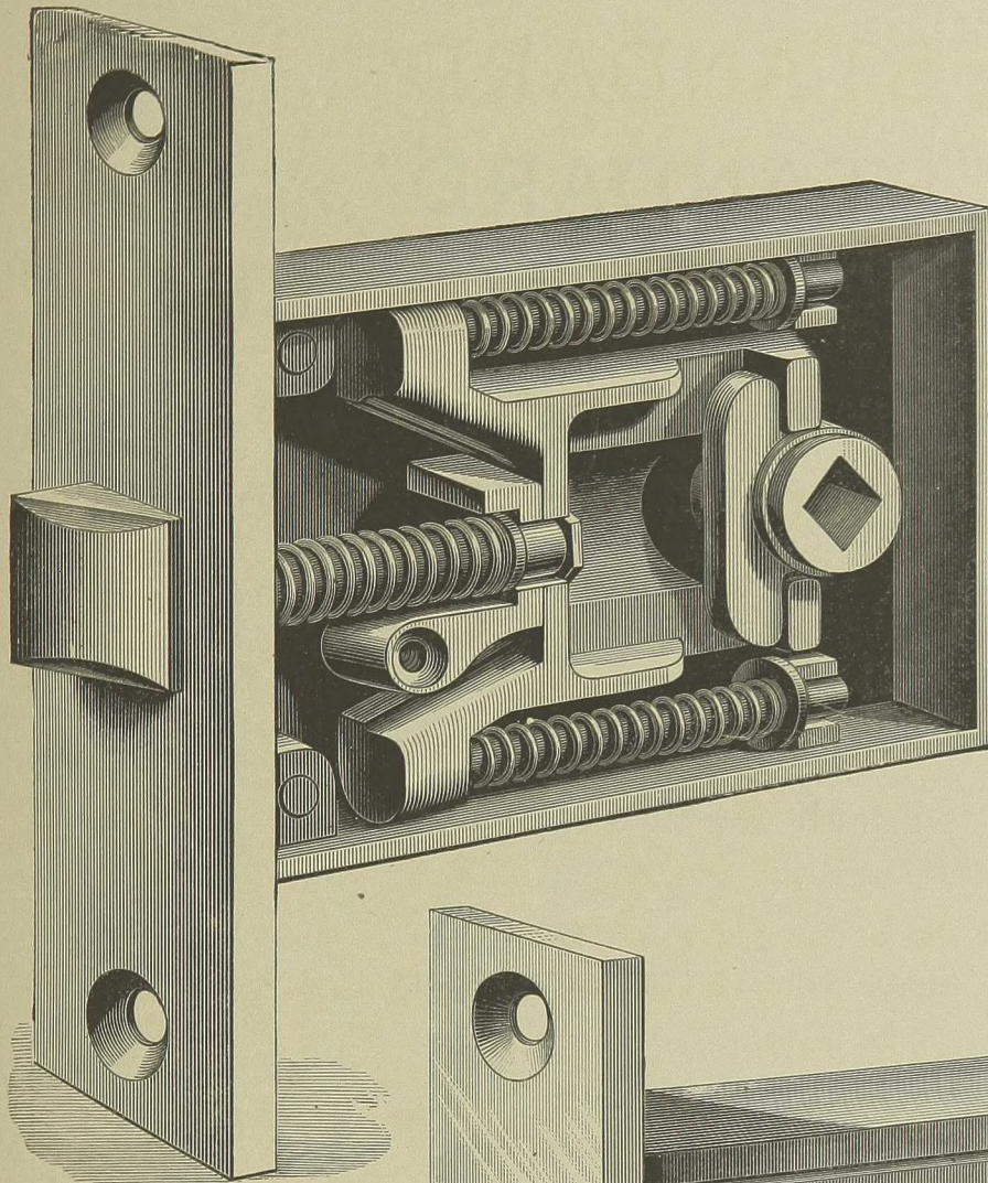
No. 1000. Standard Mortise Knob Latch.
