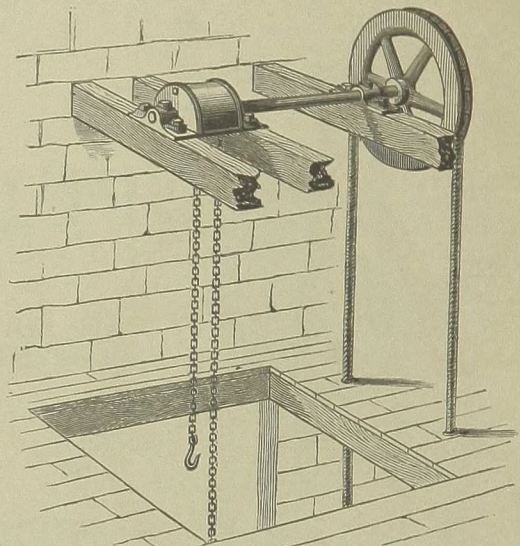
WESTON'S "DOUBLE LIFT." With Lengthened Shaft, For use over Hatchways.
