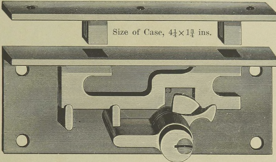
Chest Lock, No. 121.
