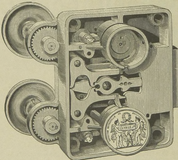
YALE DOUBLE DIAL LOCK.
