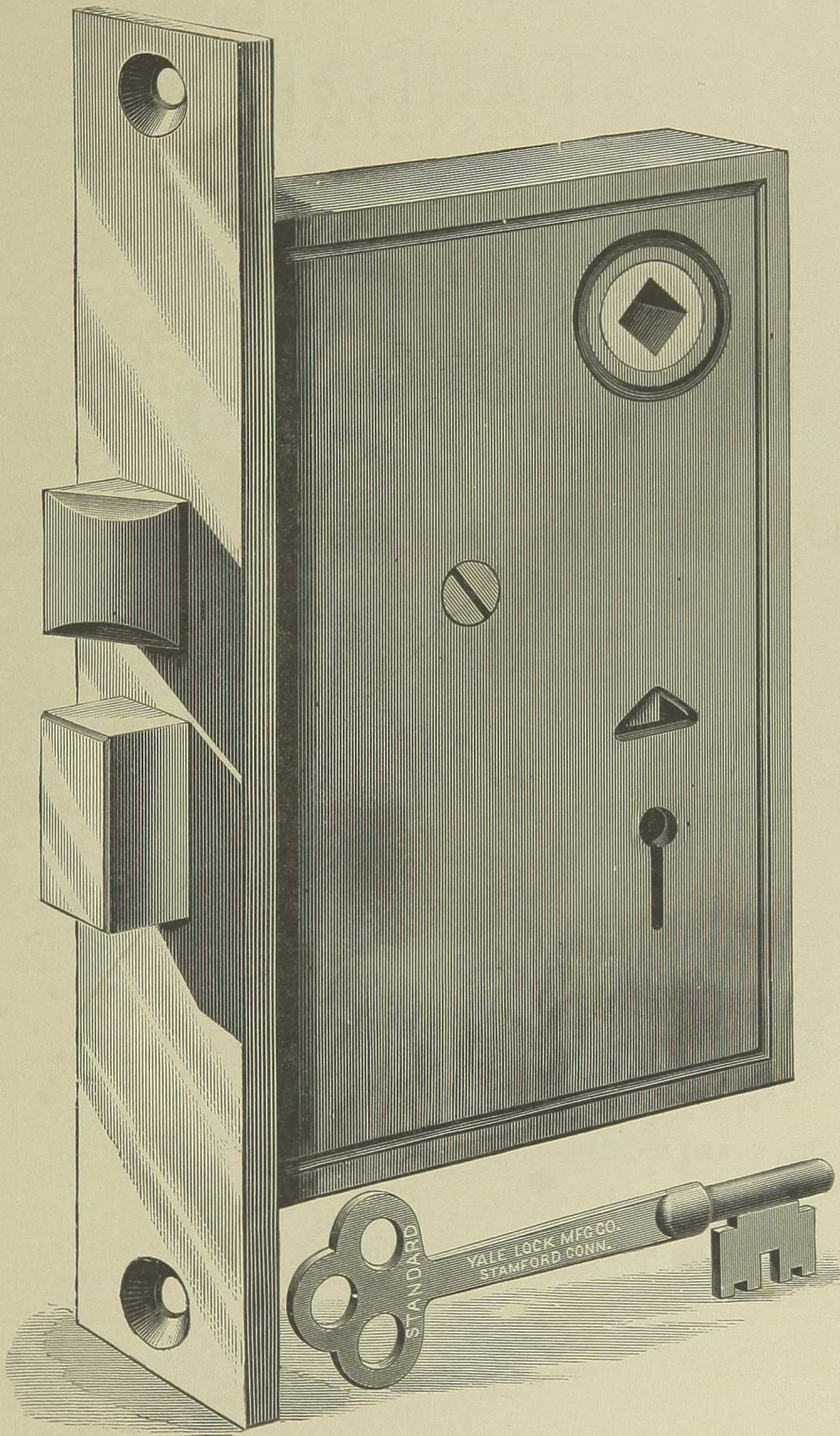
No. 1420. Standard Mortise Knob Lock. FOR NARROW STILES.
