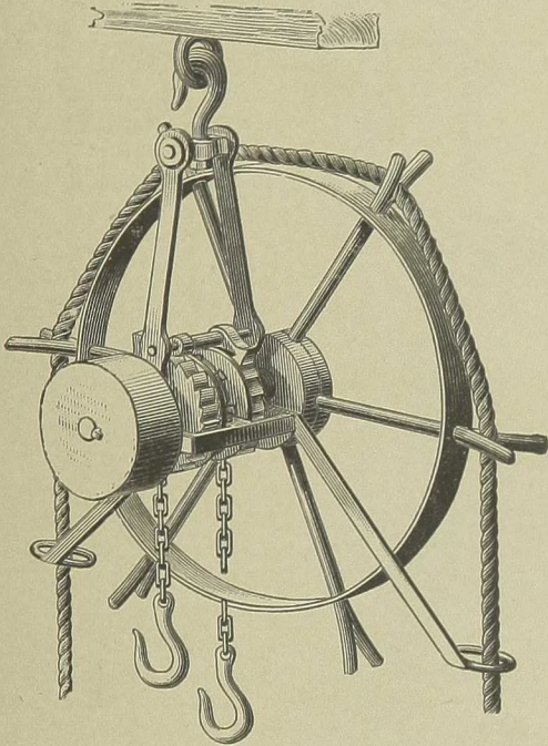
PORTABLE DOUBLE LIFT. Capacity 500 lbs.
