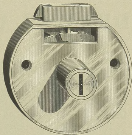
STANDARD RIM-FLUSH DESK LOCK.
