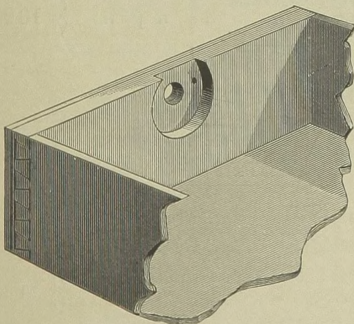
FIG. II. [Drawer Mortised ready for Lock.]
