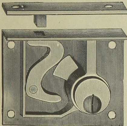
Desk Lock, No. 141.
