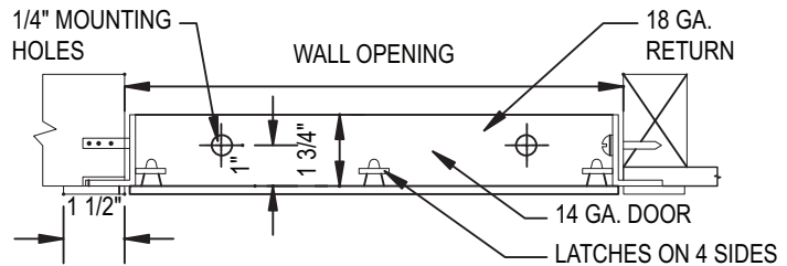
SECTION DETAIL
