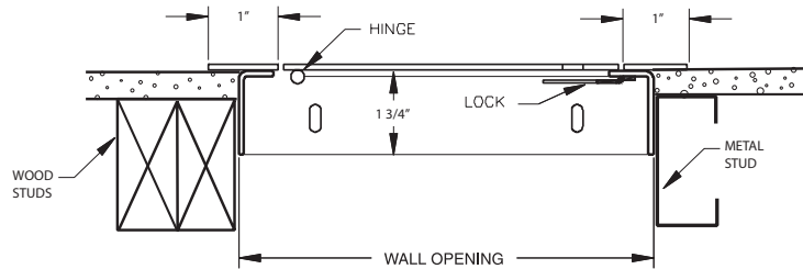
SECTION DETAIL
