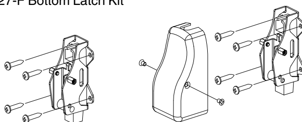
8827-F Bottom Latch Kit
