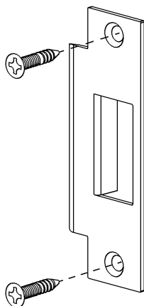
575 Mortise Strike
