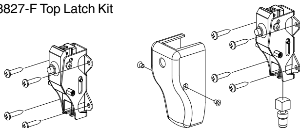
8827-F Top Latch Kit
