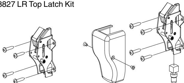
8827 LR Top Latch Kit
