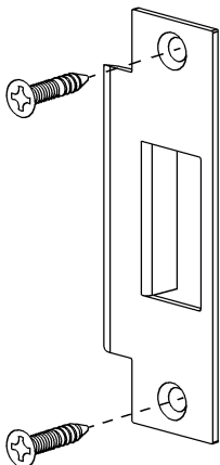
575 Mortise Strike
