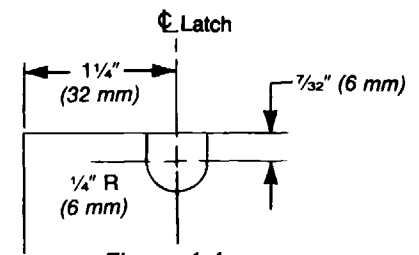
Figure 1-4 TOP OF DOOR
