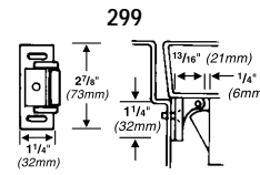
Projection 13/16" (21mm)
