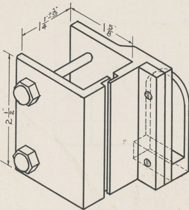
No. 2051 R.H. R.B. Clamp Keeper for Right-hand door opening out
