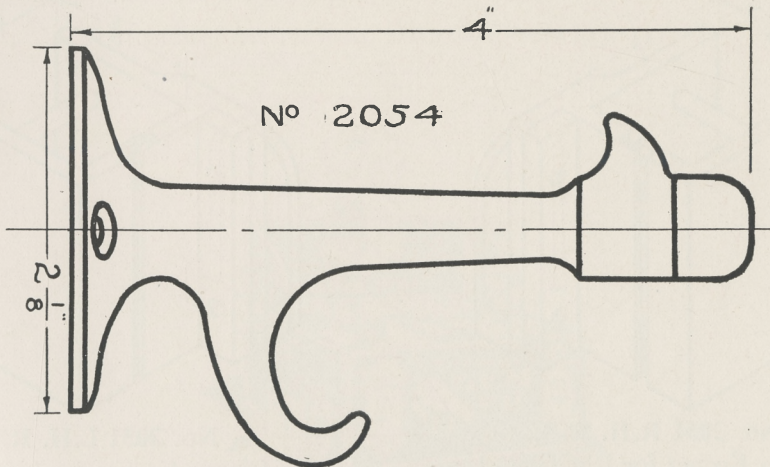
Coat Hook with Rubber Bumper
