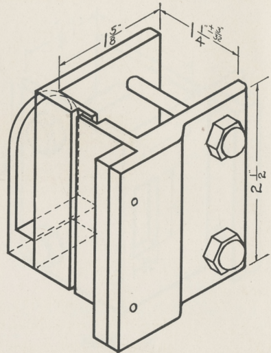
No. 2050 L.H. Clamp Keeper for Left-hand door opening in
