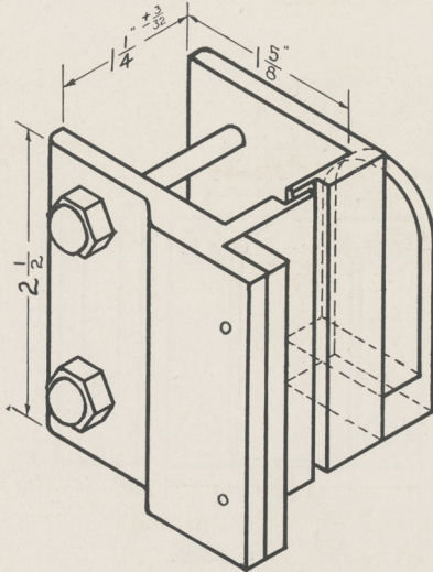
No. 2050 R.H. Clamp Keeper for Right-hand door opening in
