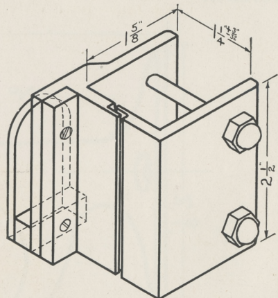
No. 2051 L.H. R.B. Clamp Keeper for Left-hand door opening out
