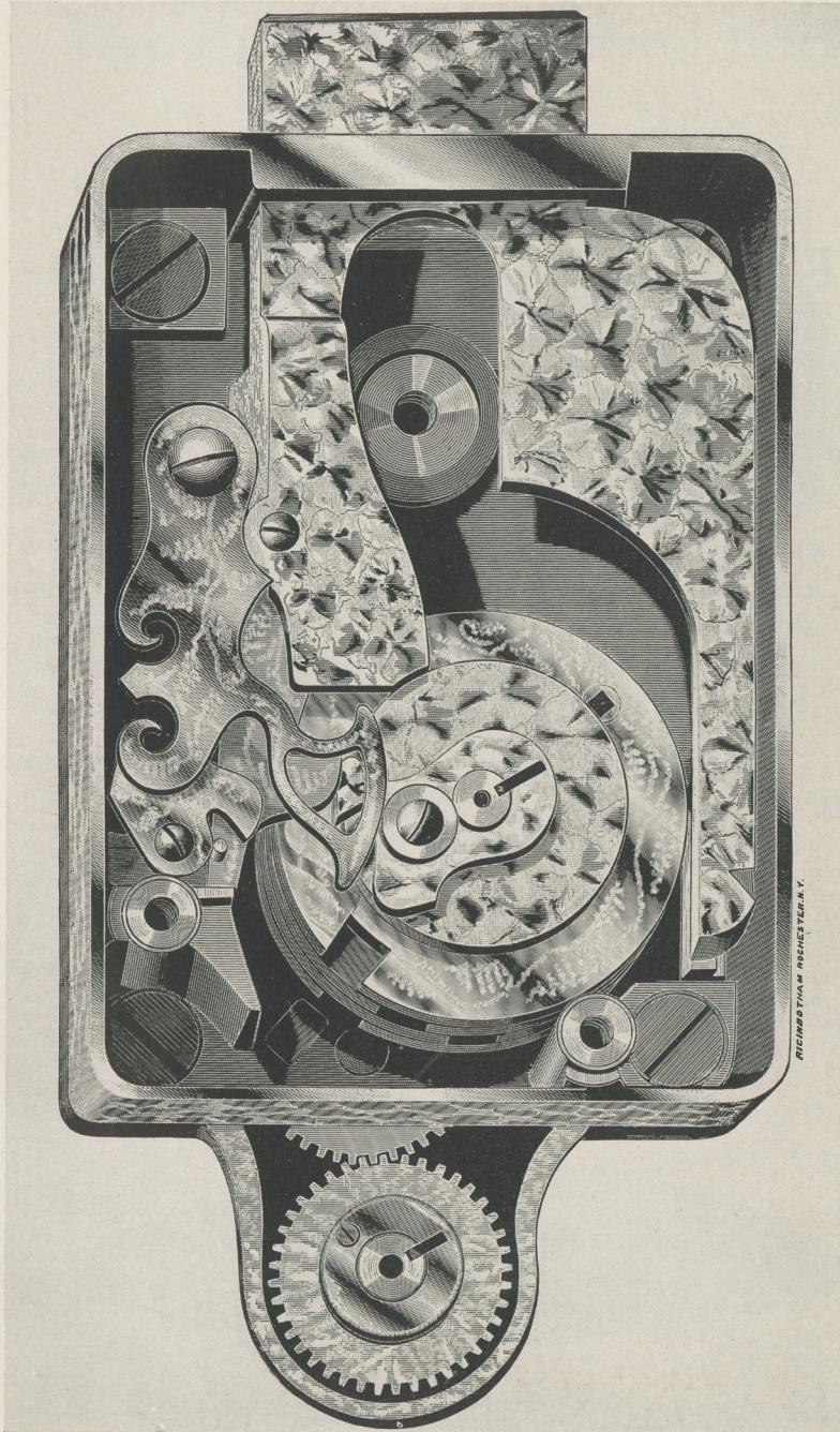
Combination Lock C-39½
