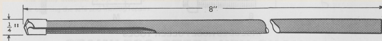
No. SHPD-12 1/4" Tungsten Tip
