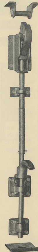
No. 3988 Self-latching End case 3¾ x 2½ in. Center case 2½ x 2½ in. Rod ½ in.
