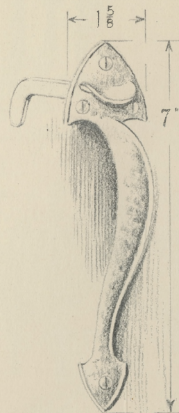
581 with Latch Bar 58178 for Lock
