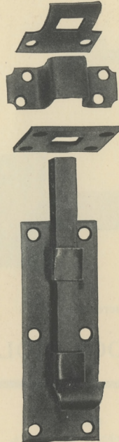
No. 9582 5¾ x 1¾ in. 1½ in. Projection
