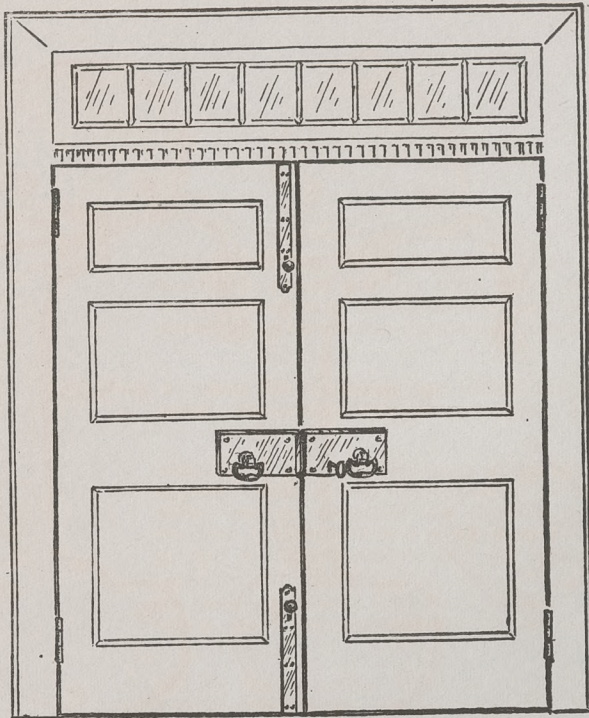
DOUBLE DOOR BALANCED WITH BOX ON EACH
