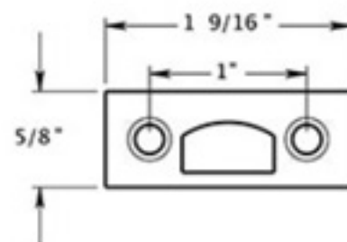
Mortise strike
