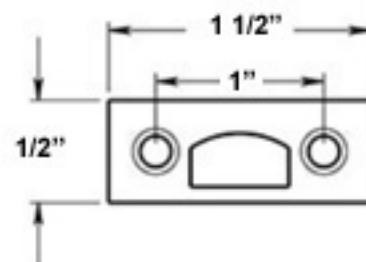
Mortise Strike
