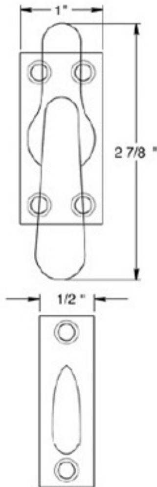
FRONT VIEW
