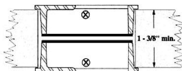
Two Pulls One Door
