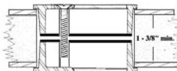
Back-to-Back Pulls for Hollow Core Doors
