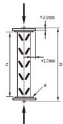
Upright Post Test
