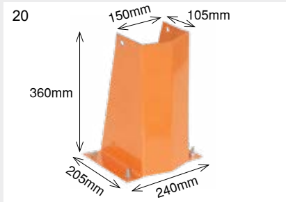
O Frame Guard (Type A)
