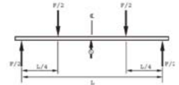
Box Beam Test
