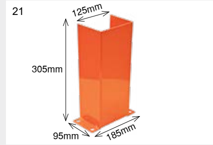
O Frame Guard (Type B)
