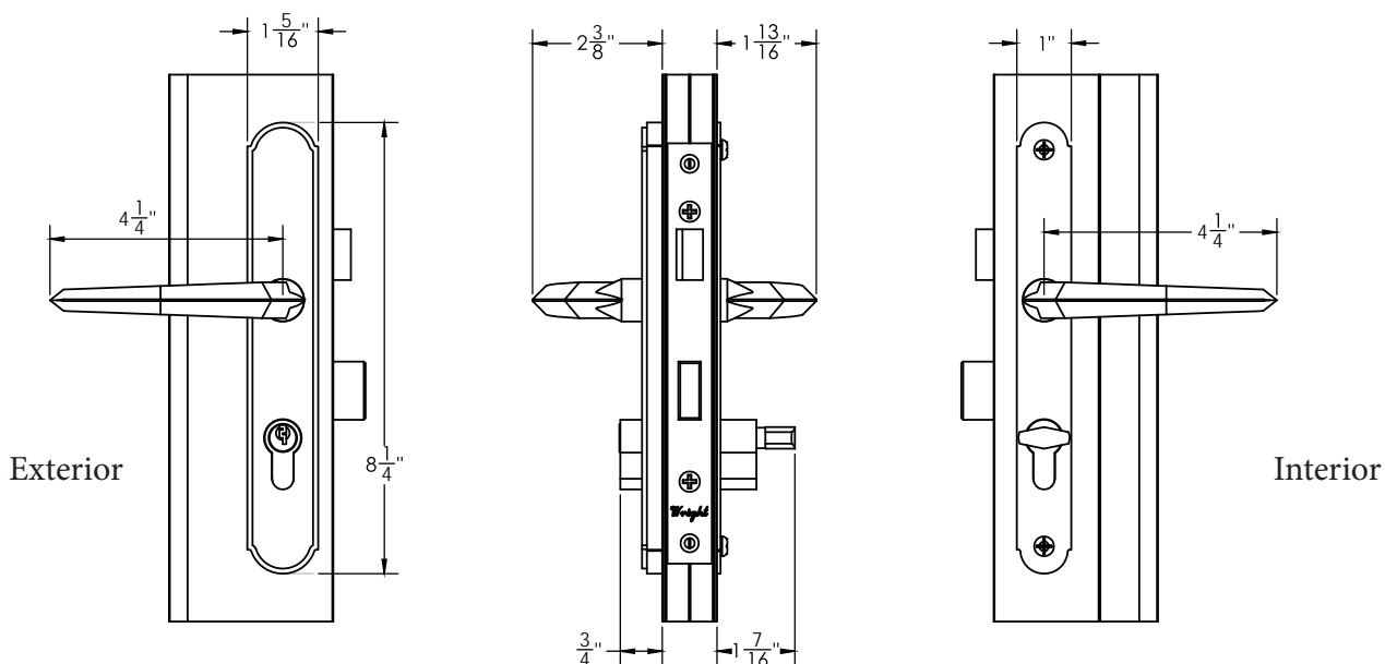
C5374BL Tru-Frame® and TruView™ Hardware Dimensions
