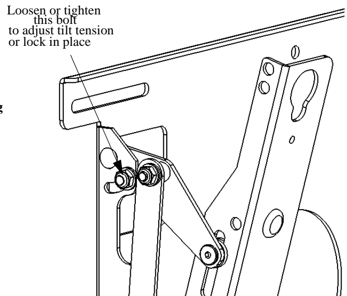
Figure 7. Tilt Tension Adjustment
