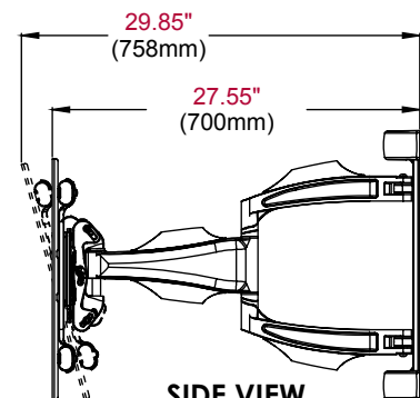
SIDE VIEW EXTENDED
