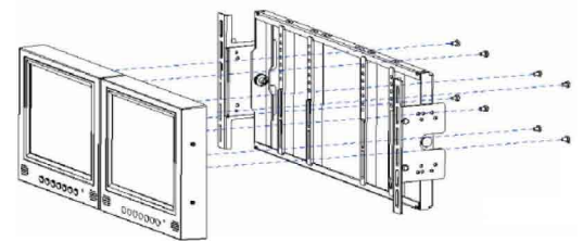
DUAL MOUNT
