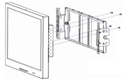
SINGLE MOUNT
