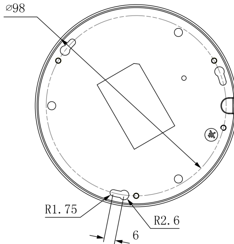
Figure 2-3 Dimension illustration 2
