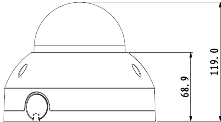
Figure 2-1 Dimension 1
