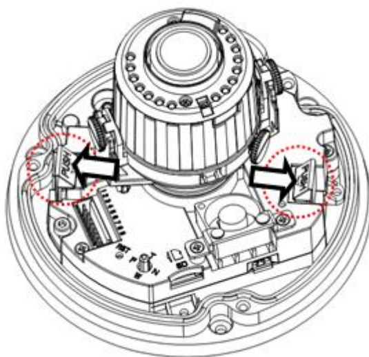
Figure 3-3 Installation 2
