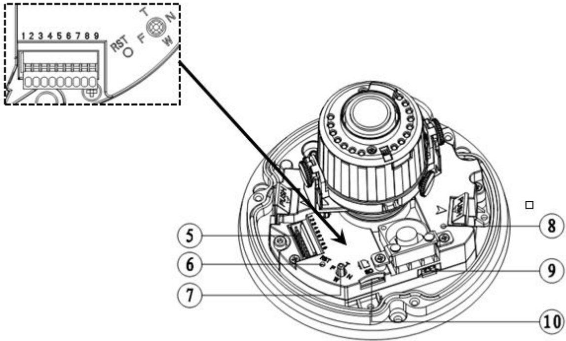
Figure 2-3 Motorized focus camera internal with IR (1-a)
