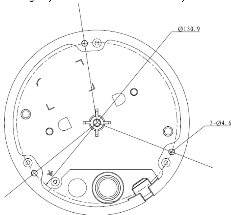
Figure 3-1 Installation 1
