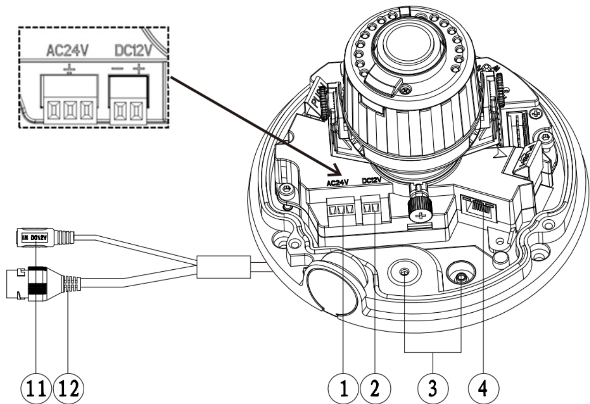
Figure 2-4 Motorized focus camera internal with IR (1-b)
