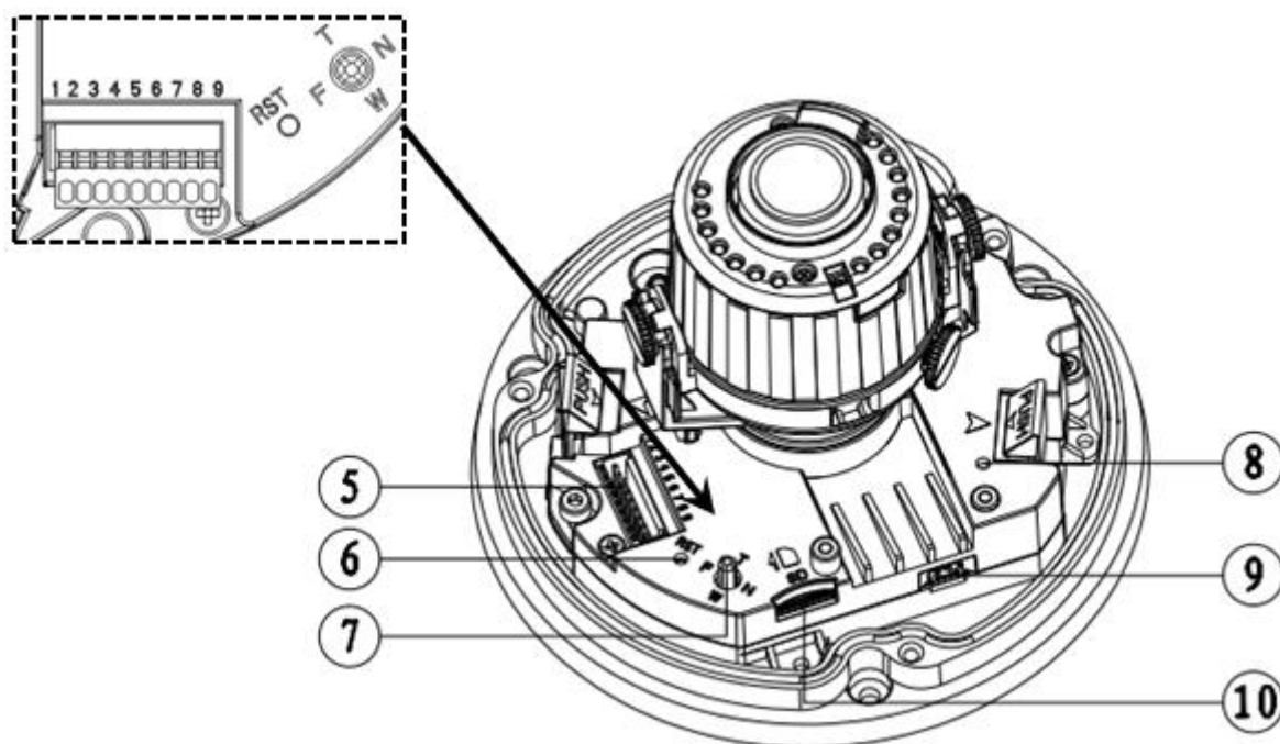
Figure 2-5 Motorized focus camera internal with IR (2)
