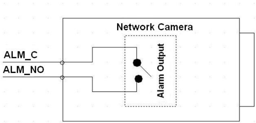
Figure 2-8 Alarm output
