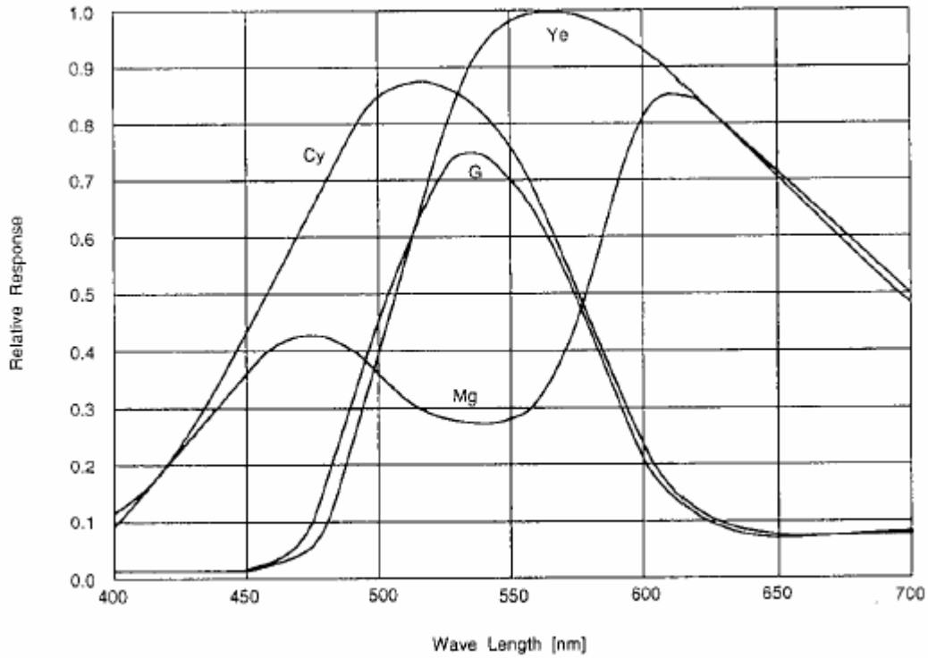
KP-D20A/B R2 Version Spectral Response with Lens
