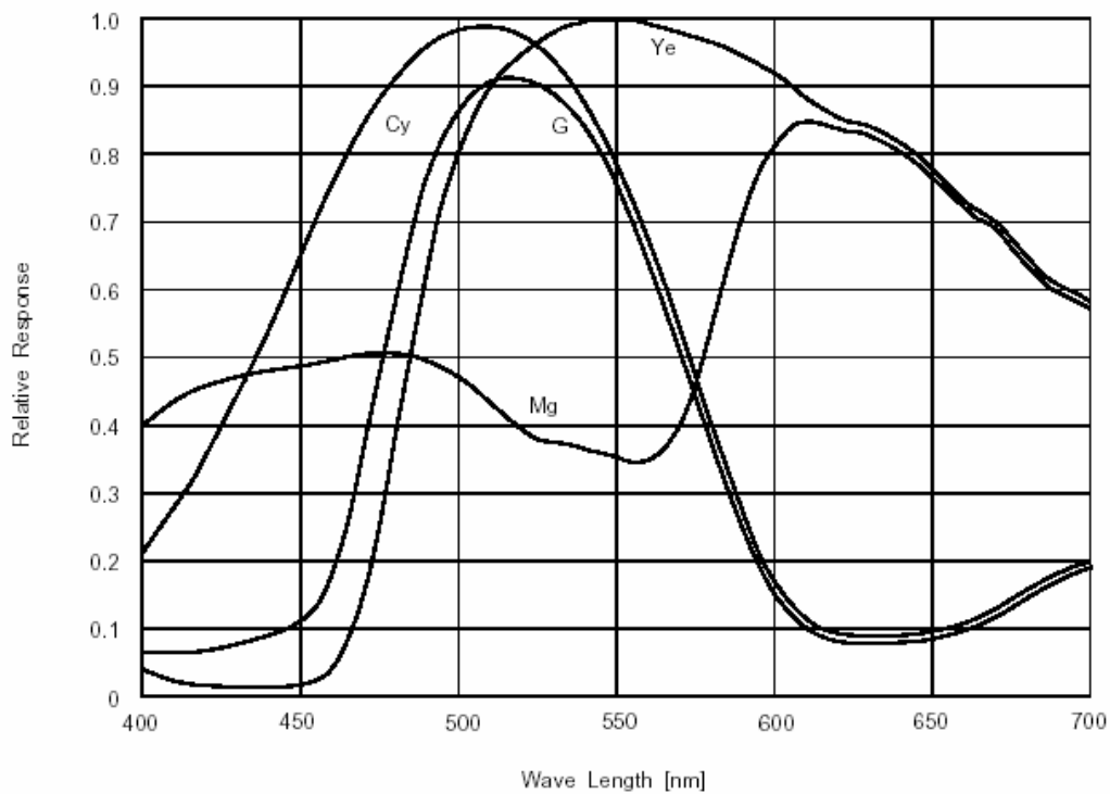
KP-D20A/B R3 Version Spectral Response with Lens
