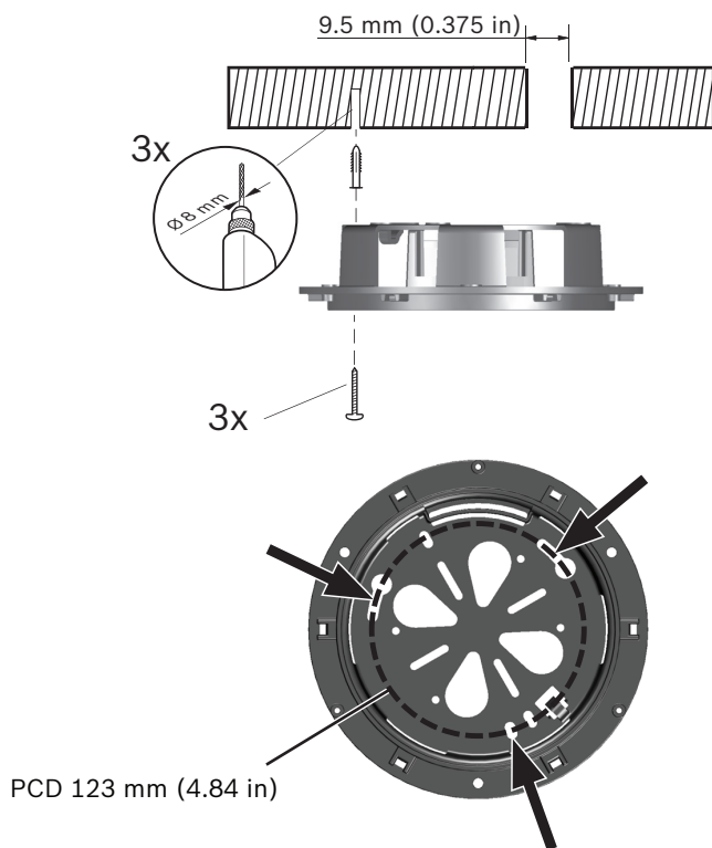
Figure 5.1 Surface mounting
