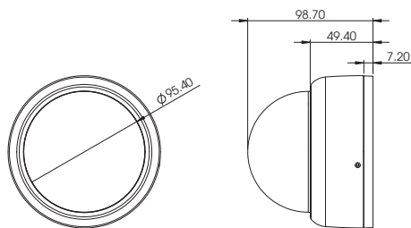
Indoor Dome Dimensions
