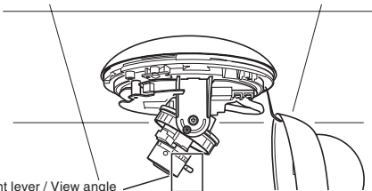
Focus adjustment lever / View angle adjustment lever
