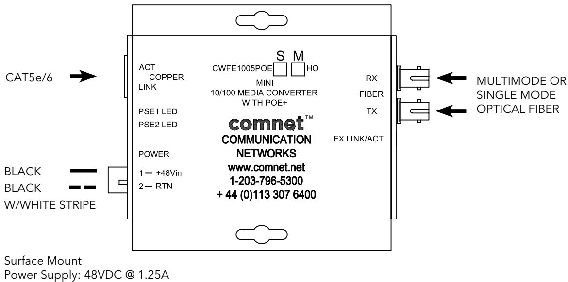
FIGURE 7 - CWFE1005POE(M,S)HO-M MEDIA CONVERTER
