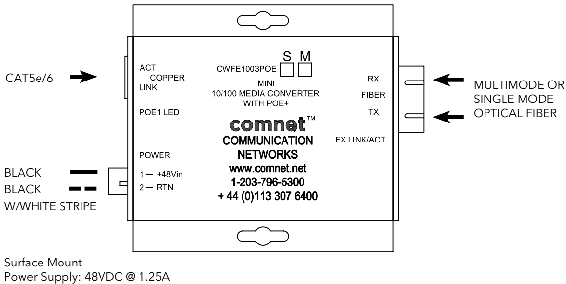
FIGURE 1 - CWFE1003POE(M,S)-M MEDIA CONVERTER
