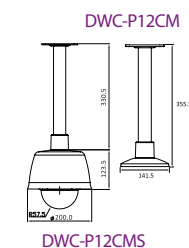
DWC-P12CMS
