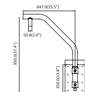
DWC-P39PARAM
