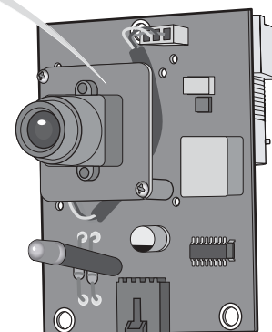
Camera Module Replaces the LED Board.
