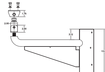
Corner Mount Side View ADCHMTCRNR
