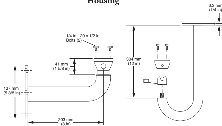
Wall Mount Side View ADCHMTWALL
