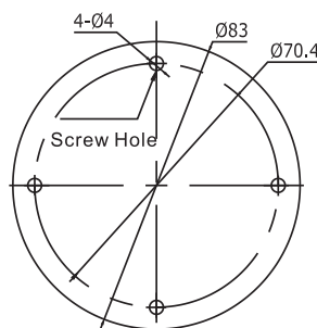
Figure 2-6 Drill Template
