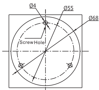
Figure 2-1 Drill Template
