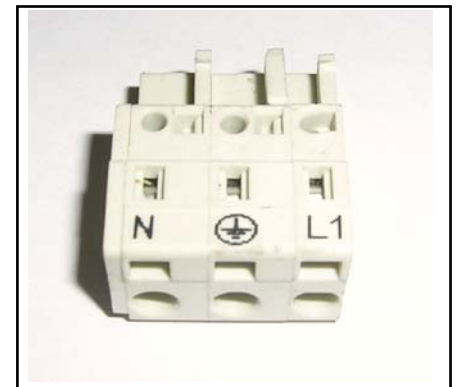
140676 MAINS PLUG
