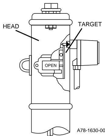
Falling flag
