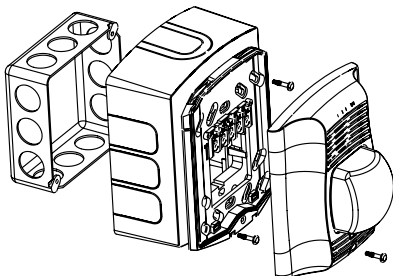
FIGURE 6. WALL MOUNT PRODUCT WITH BACK BOX SKIRT:
