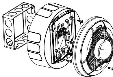
FIGURE 8. WALL MOUNT HORN/STROBE WITH WEATHERPROOF BACKBOX:
