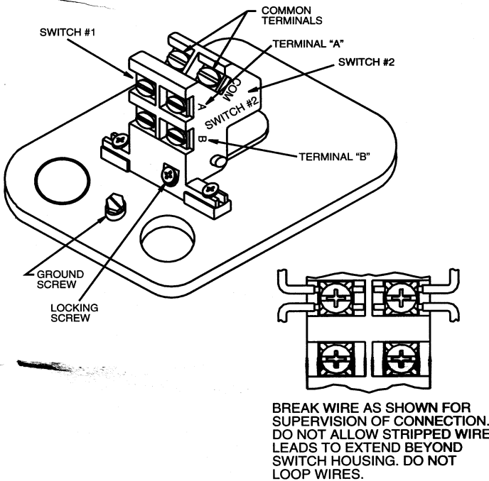
Figure 3. Switch terminals:
