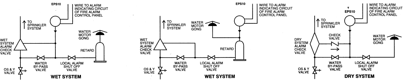
Figure 2. Typical piping diagram for EPS10-1, EPS10-2
