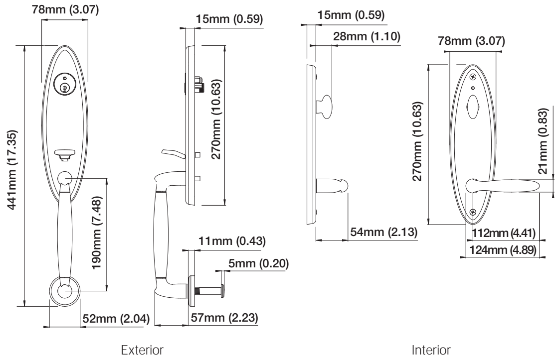
Entry Set Shown
