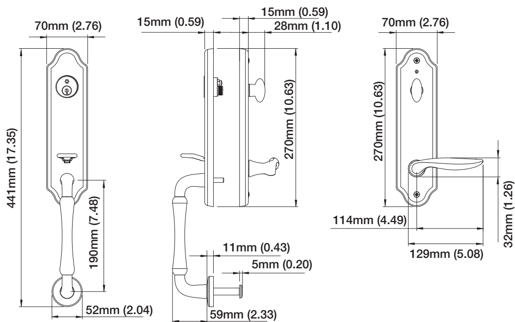
Exterior
