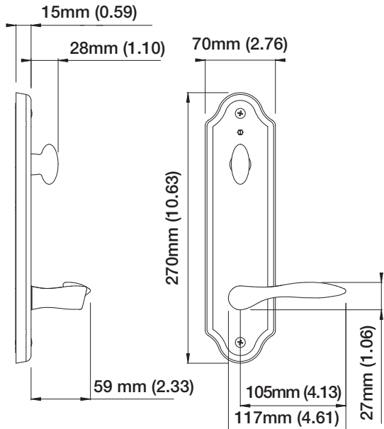
Interior
