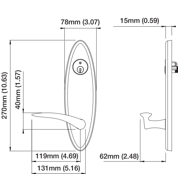
Exterior
