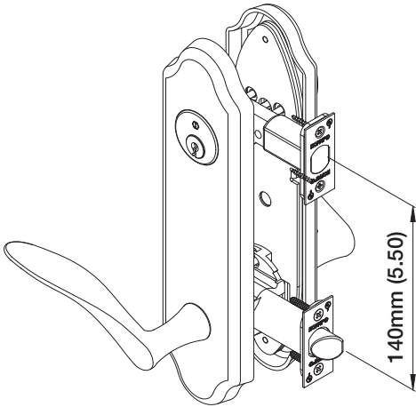
Entry Set LH Shown
