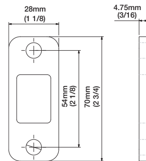
Underplate For T-Latch Strike
