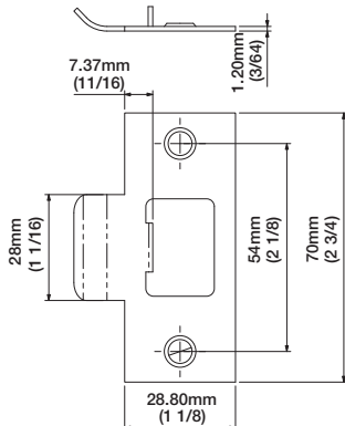
T-Latch Strike
