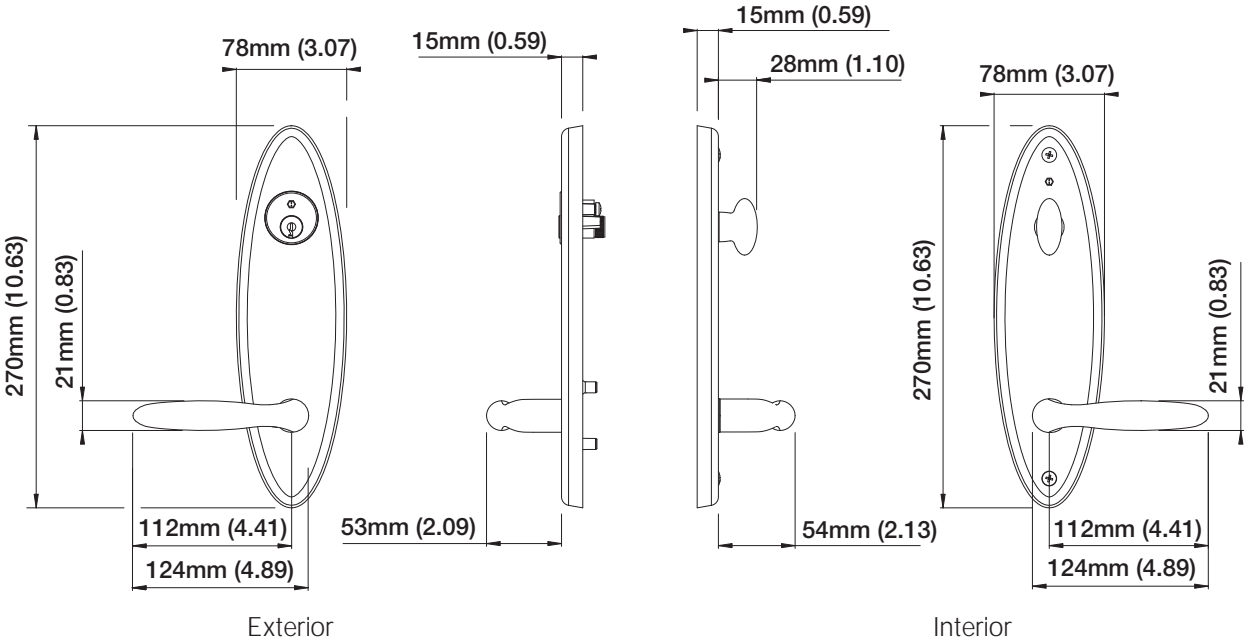
Entry Set Shown
