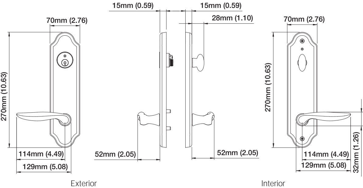
Entry Set LH Shown
