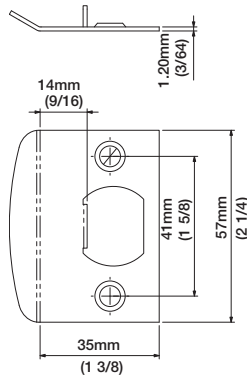
Full Lip Latch Strike
