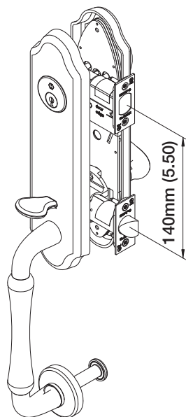
Entry Set LH Shown
