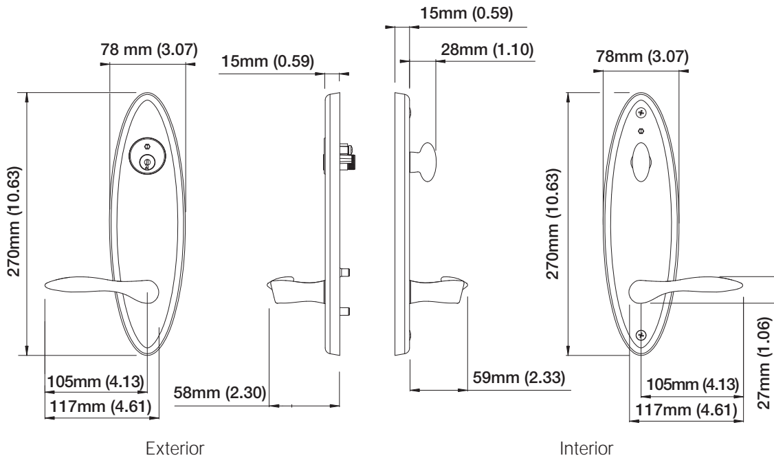
Entry Set LH Shown
