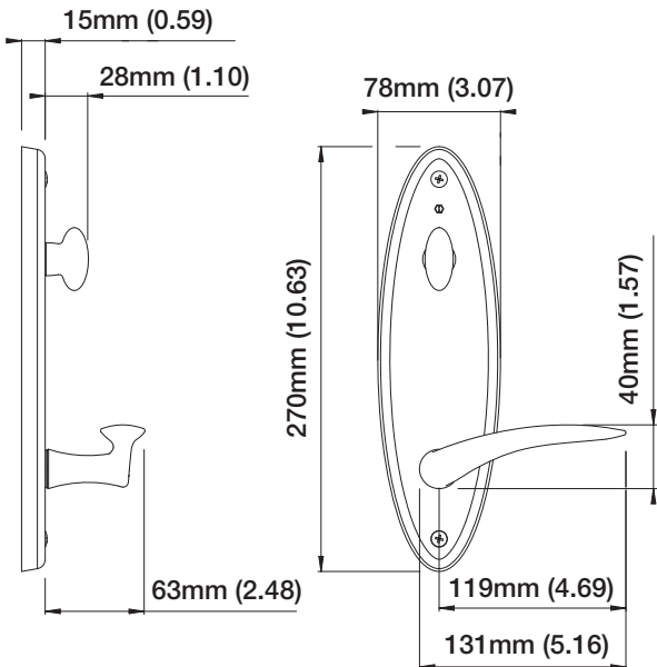
Interior
