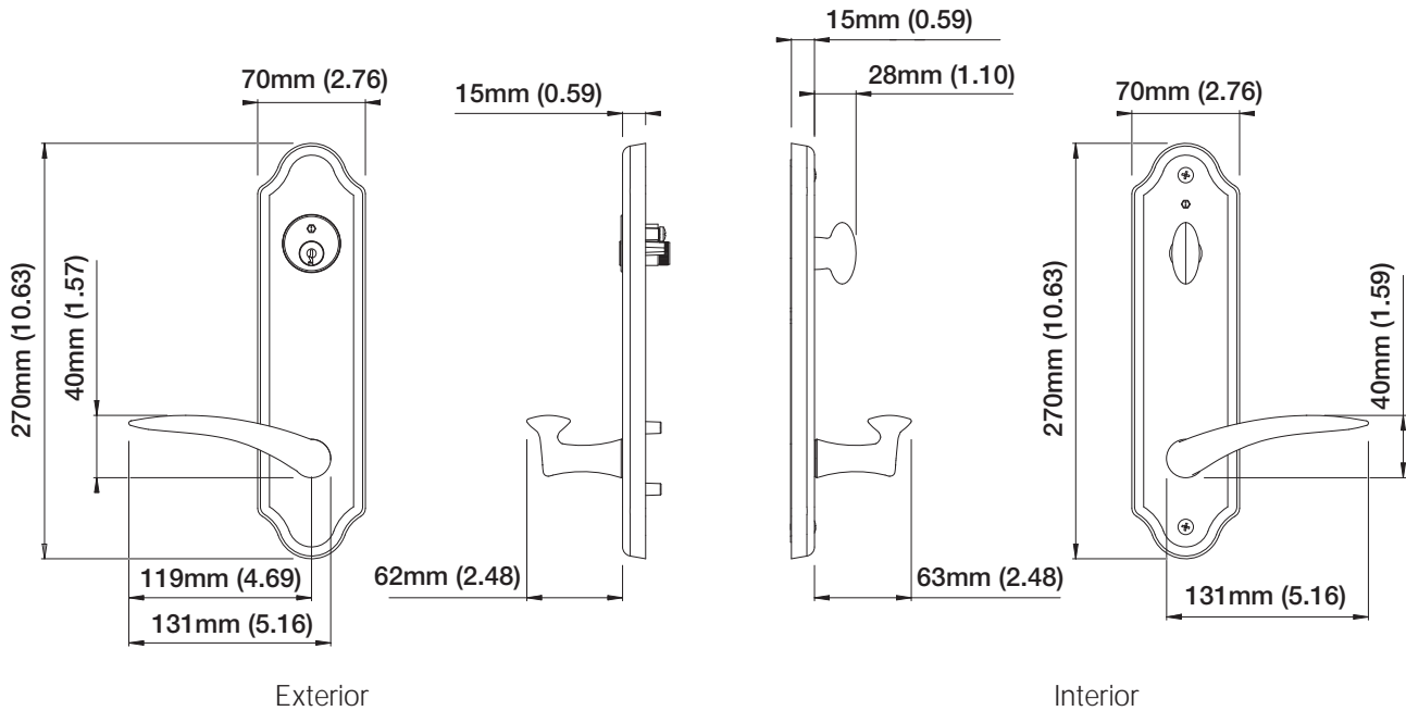
Entry Set LH Shown
