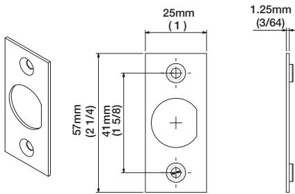
Latch Faceplate Pack Includes both Radius and Square Cornered Faceplates and Screws
