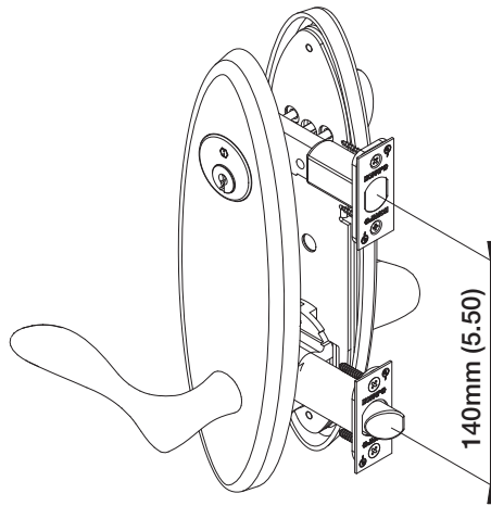
Entry Set LH Shown
