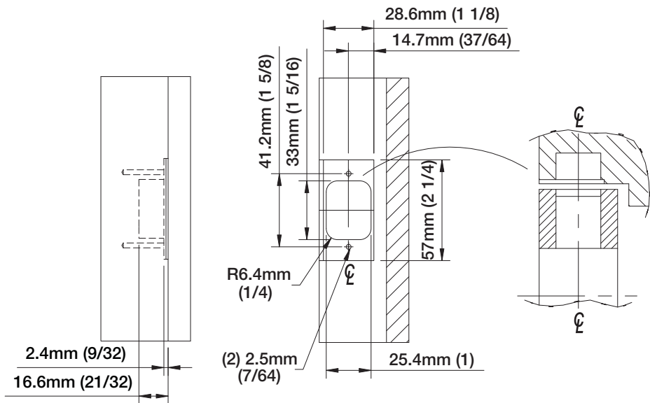
Strike Prep
