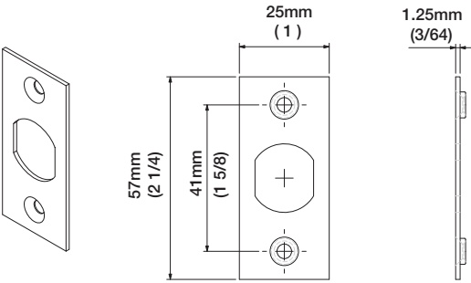
Deadbolt Faceplate Pack Includes both Radius and Square Cornered Faceplates and Screws
