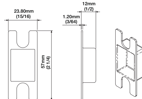
Dustcap For Latch Strike
