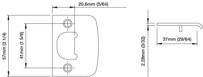
Full Lip Latch Strike Packs Include Square Cornered Strikes and Screws
