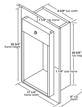
SEMI-RECESSED 100-SR (5 LB.) OUTSIDE DIMENSIONS
