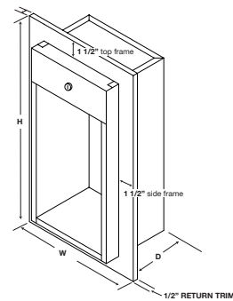
SEMI-RECESSED 999-SR (10 LB) ROUGH OPENING DIMENSIONS
