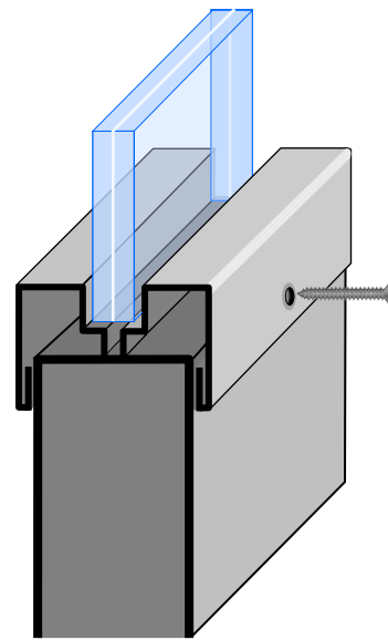
ALK-3 1-3/4" Metal Door All Single Glass Configurations
