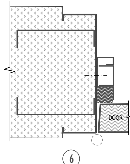
6 Pour-in-Place Installation in New Concrete Wall
