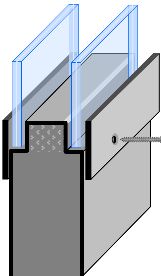
ALK-2 (STD) 1-3/4" Metal Door All Dual Glass Configurations
