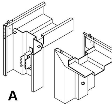
OPPOSITE VIEWS OF CORNER MITRE
