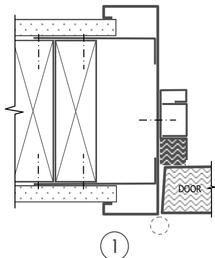
1 Nail-in Installation in Wood Stud Wall
