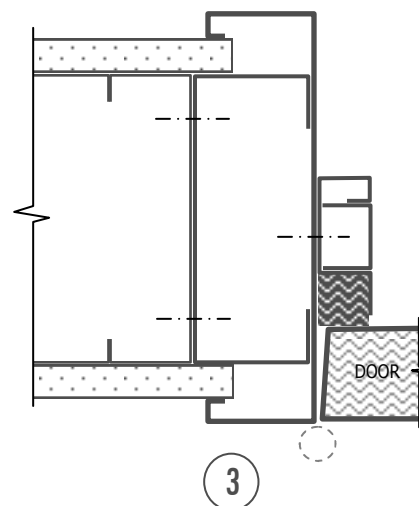
3 Built-in Installation in Steel Framed Wall
