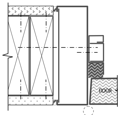
2 Bolt-in Installation in Existing Wood Stud Wall
