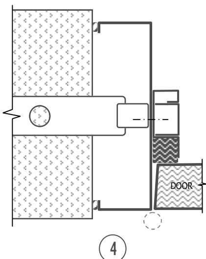
4 Built-in Installation in New Masonry Wall
