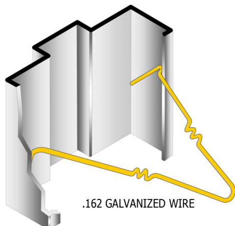
T-9 MASONRY ANCHOR
