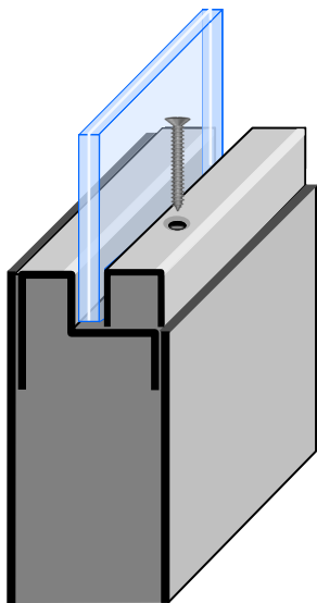
ALK-1 (STD) 1-3/4" Metal Door Up to 5/8" Single Glass Configurations
