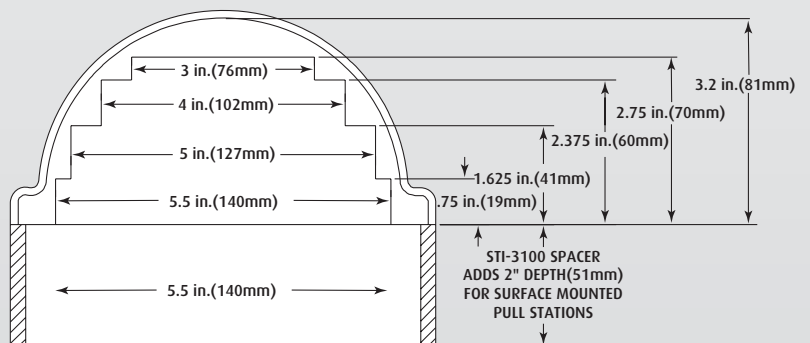
ALL MODELS END VIEW
