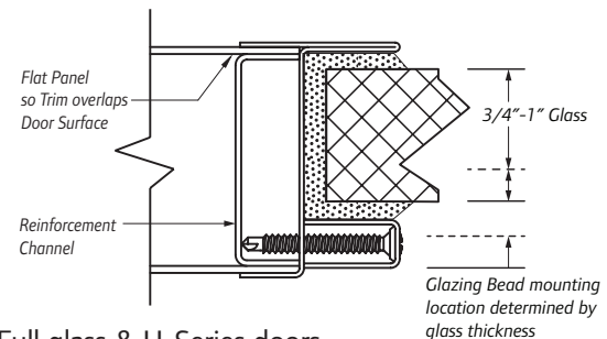
Overlapping Steel Trim for 3/4" THRU 1" Insulated Glass
