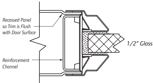
Designer® Trim (recessed) for 1/2" Insulated Glass
