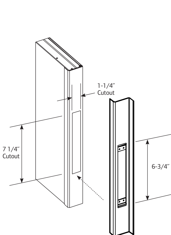
Astragal attachment Detail
