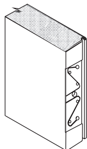
Universal Mortise Hinge 7 Gage Universal hinge reinforcement
