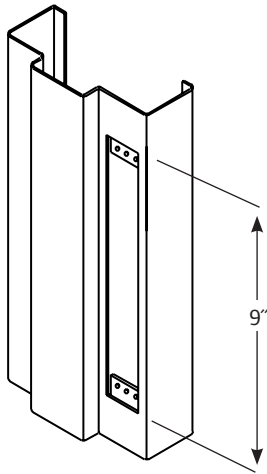
Typical Frame Preparation
