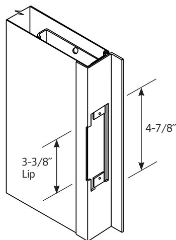
Final Assembly Detail
