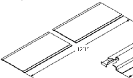
Filler Plate without Stop TSF-27
