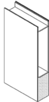
Standard 14 Gage [0.067" (1.7mm)] Closer Reinforcement
