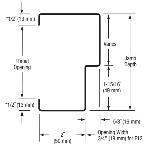
Single Rabbet Frame
