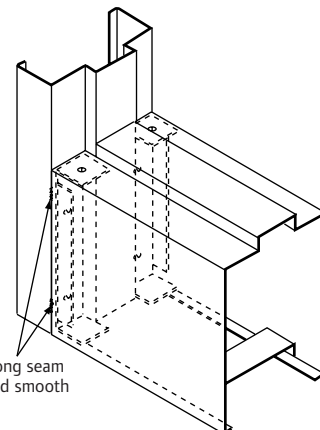
Detail 3 Sill Connection
