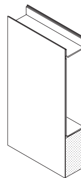
Optional 14 Gage [0.067" (1.7mm)] Closer Reinforcement
