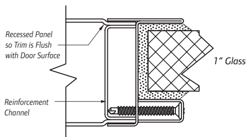
Flush Mounted Steel Trim for 1" Insulated Glass
