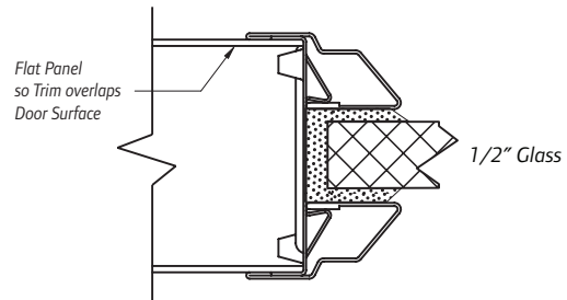
Designer® Trim (for Distributor Prep) for 1/2" Insulated Glass
