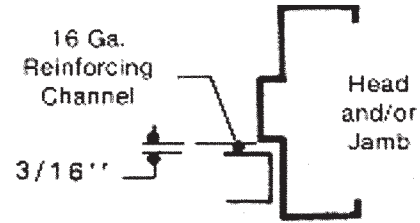
TYPICAL CHANNEL LOCATION
