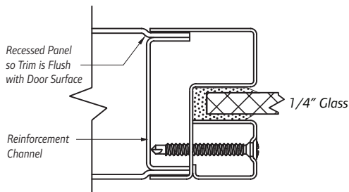
Flush Mounted Steel Trim for 1/4" Glass
