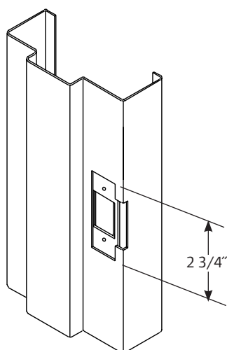
Typical Preparation
