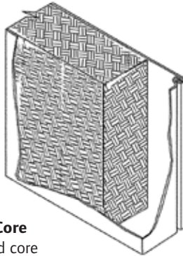
Mineral Board
