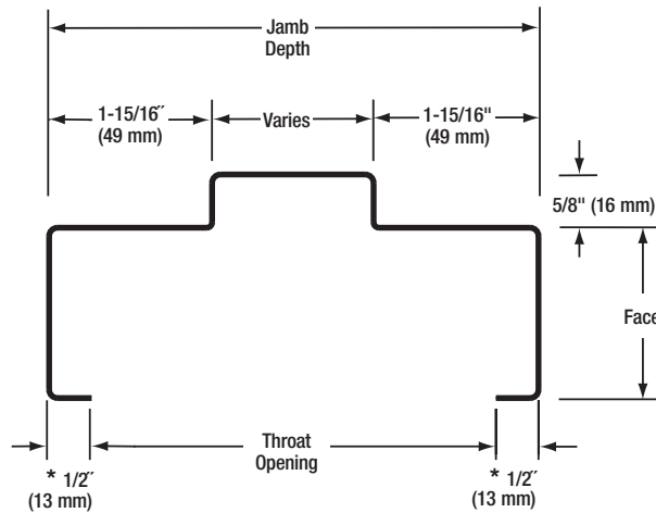
Standard Double Equal Rabbet Frame
