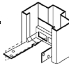
DW-Series Adjustable Lock-in Base Anchor - Refer to page 2.4.14
