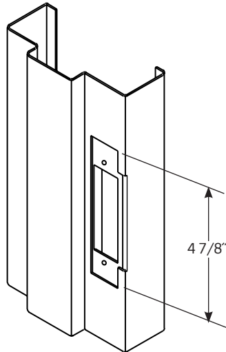
Typical Preparation
