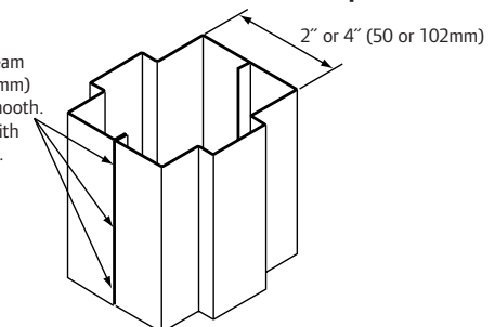
Detail 6 – Double Frame Section Option
