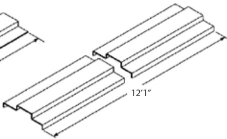
Multi-use Filler Plate with Stop TSF-95
