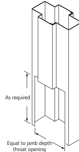
Detail 4 – Closed Section (with partial side light option)
