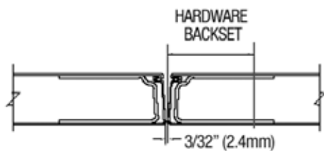
Without Astragal
