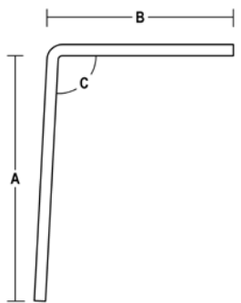
K44 93° SURFACE EDGE GUARD - HALF
