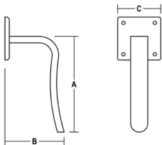
H417 ARM PULL W/ SQUARE BASE
