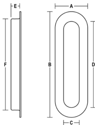
H472 OVAL FLUSH PULL W/ CONCEALED MOUNTING
