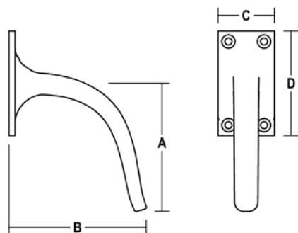
H419 ARM PULL W/ RECTANGULAR BASE
