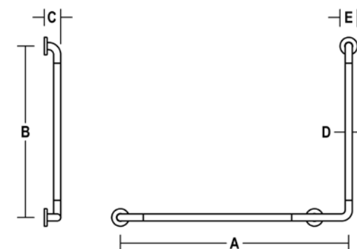
G240-70-P 40" X 30" X 90° X GRAB BAR - Ø 1-1/4"
