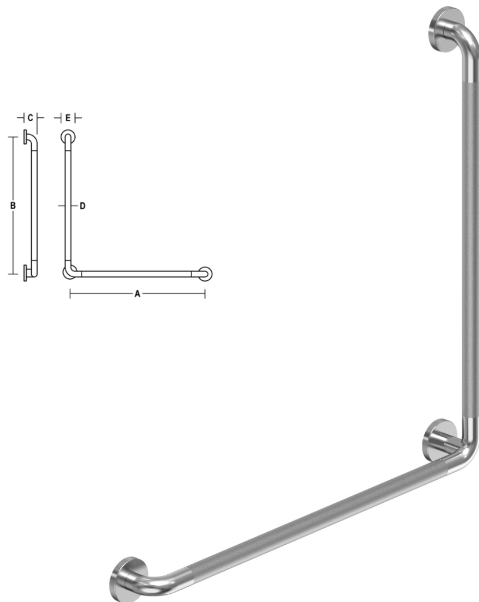
G319-70-P 36" X 36" X 90° GRAB BAR - Ø 1-1/2"
