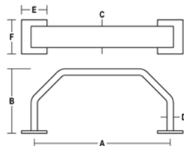
B320 HEAVY DUTY TRIM GUARD - 3.75" PROJ
