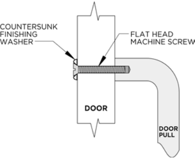
#2 = STANDARD SINGLE THRU BOLT MOUNTING FOR WOOD AND METAL DOORS
