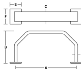
B321 HEAVY DUTY TRIM GUARD - 4.25" PROJ
