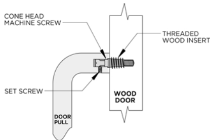
#6W = SINGLE CONCEALED MOUNTING FOR WOOD DOORS
