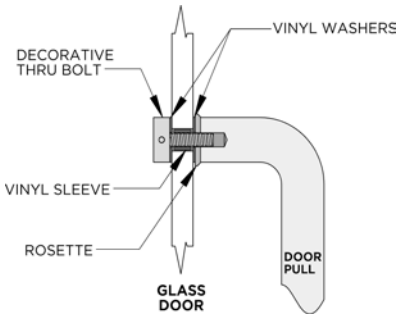
#4G = SINGLE DECORATIVE MOUNTING FOR GLASS DOORS
