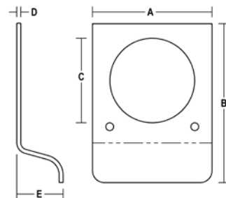
H411 Ø 2-1/8" SQUARE CYLINDER PULL
