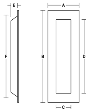
H462 6" MODERN RECTANGULAR FLUSH PULL
