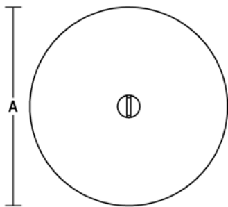
T63 CUT-OUT FILLER PLATE - FOR 2-1/8" HOLE
