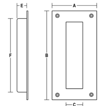
H429 TALL RECTANGULAR FLUSH PULL
