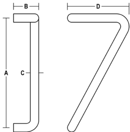
D403 ANGLED GRIP PULL
