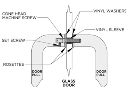
#5G = BACK TO BACK MOUNTING FOR GLASS DOORS
