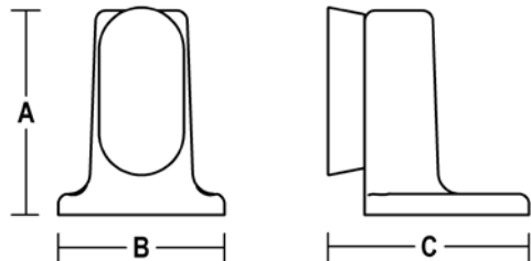
S142 HEAVY DUTY FLOOR STOP NO. A B C S142 1.625" 1.75" 2.5"
