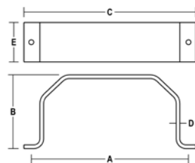
B323 STANDARD DUTY TRIM GUARD - 3.75" PROJ
