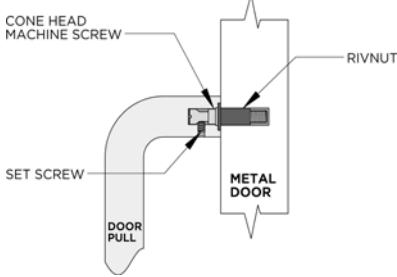
#6M = SINGLE CONCEALED MOUNTING FOR METAL DOORS
