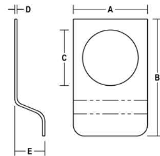
H410 Ø 1-1/2" SQUARE CYLINDER PULL
