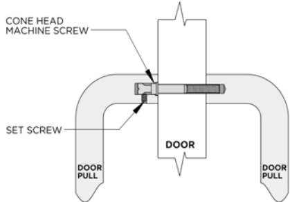
#5 = BACK TO BACK MOUNTING FOR WOOD AND METAL DOORS
