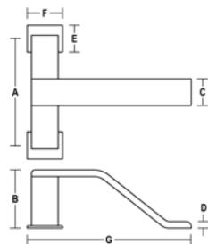
B325 HEAVY DUTY EXIT DEVICE GUARD - 3.25" PROJ
