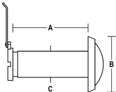
F93 DOOR VIEWER W/ PRIVACY COVER
