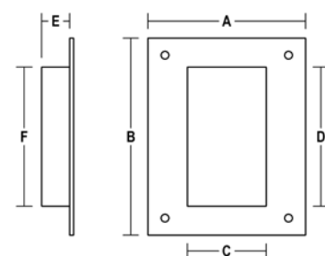
H406 RECTANGULAR FLUSH PULL
