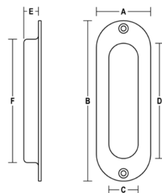
H428 OVAL FLUSH PULL
