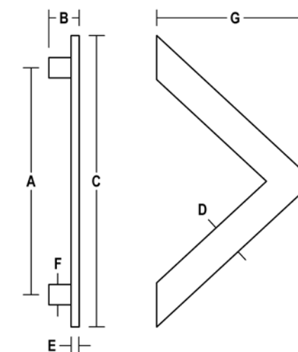
D388 RIGHT ANGLE FLAT GRIP PULL
