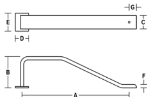
B318 12" HEAVY DUTY TRIM GUARD
