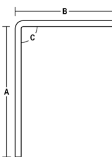
K43 90° SURFACE EDGE GUARD - HALF
