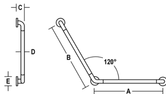
G220-70-P 24" X 24" X 120° GRAB BAR - Ø 1-1/4"
