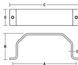
B322 STANDARD DUTY TRIM GUARD - 3.25" PROJ
