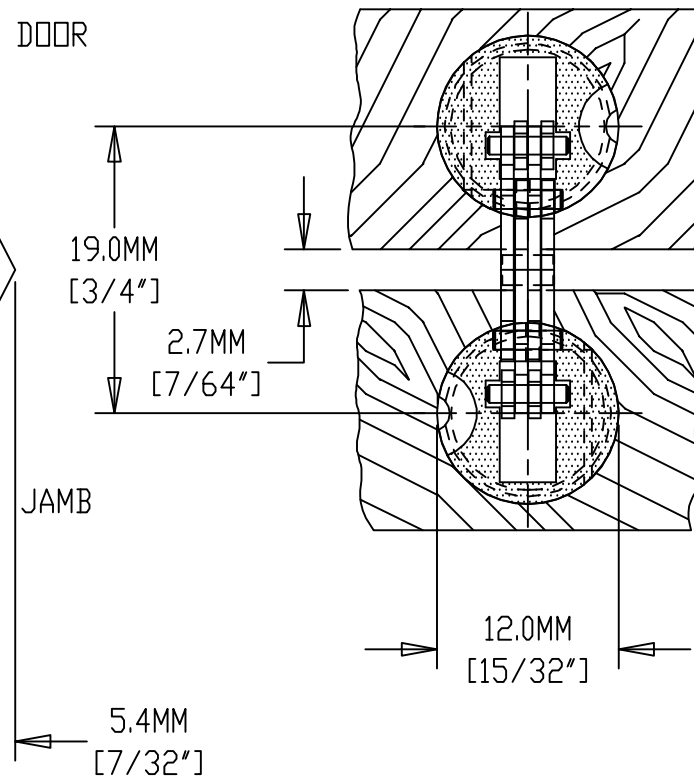
HINGE OPEN 180° FRONT VIEW
