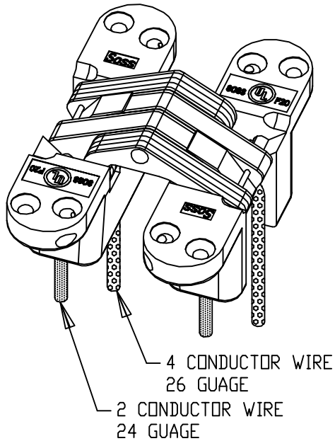
HINGE OPEN 180° ISOMETRIC VIEW
